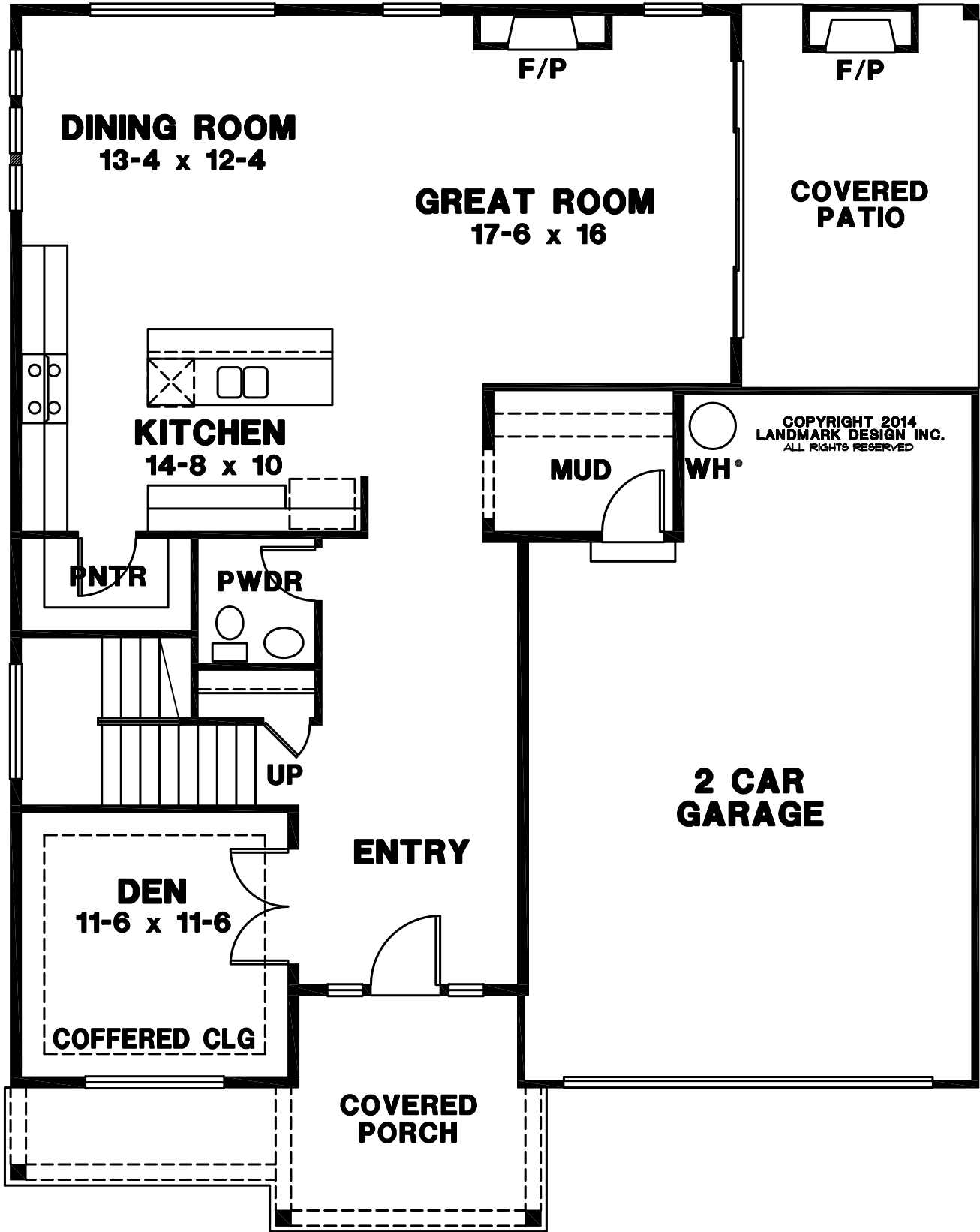
MAIN FLOOR
