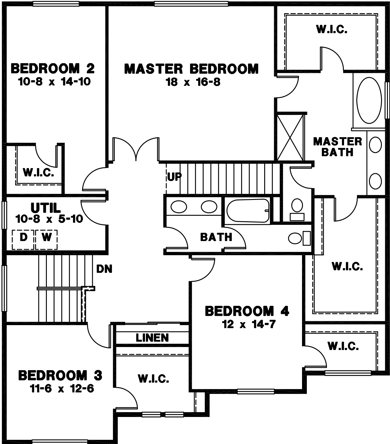
UPPER FLOOR
