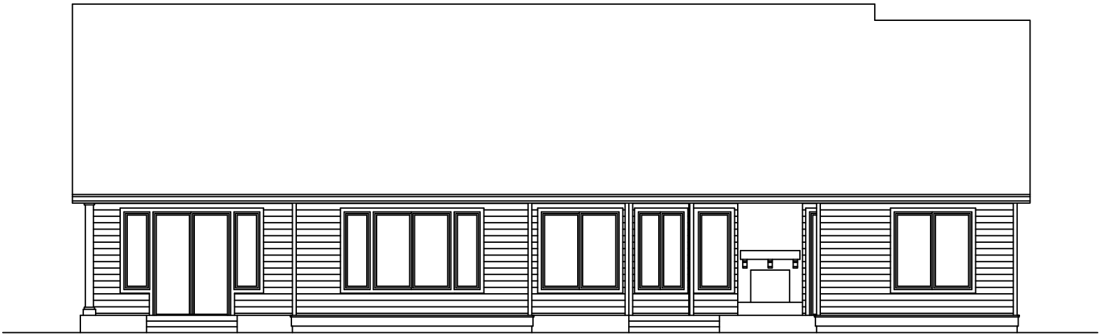
REAR ELEVATION
