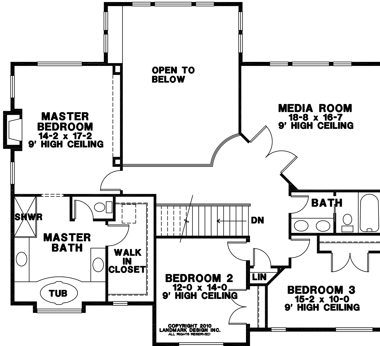
UPPER FLOOR
