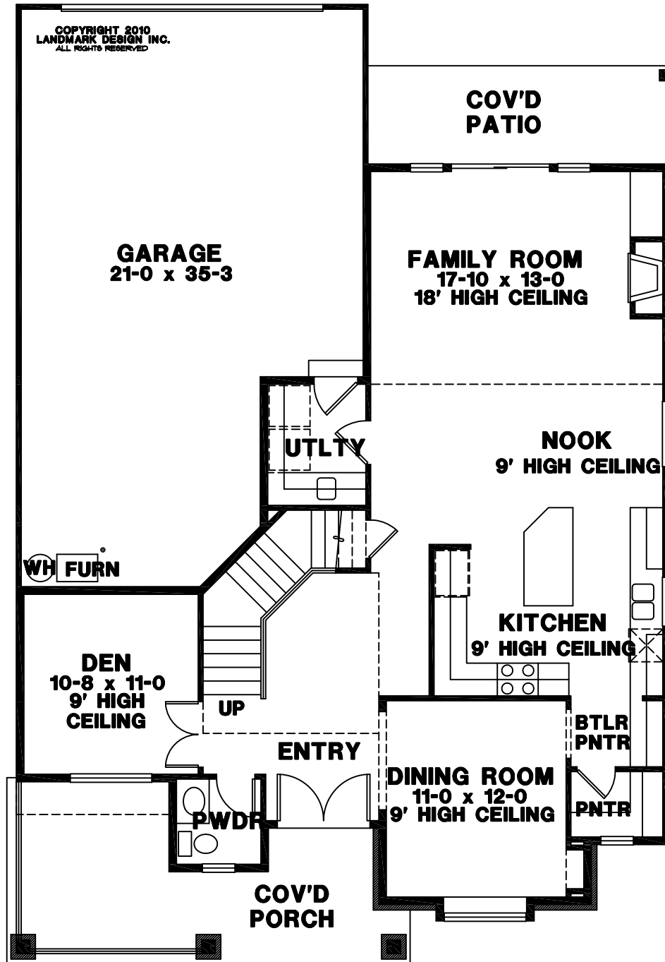
MAIN FLOOR
