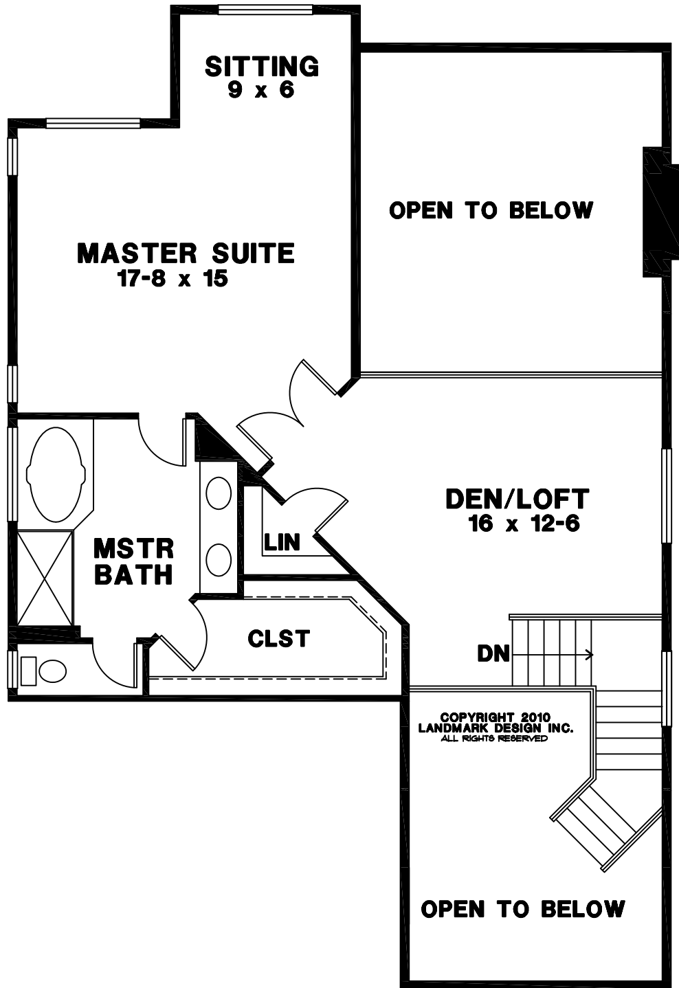
UPPER FLOOR
