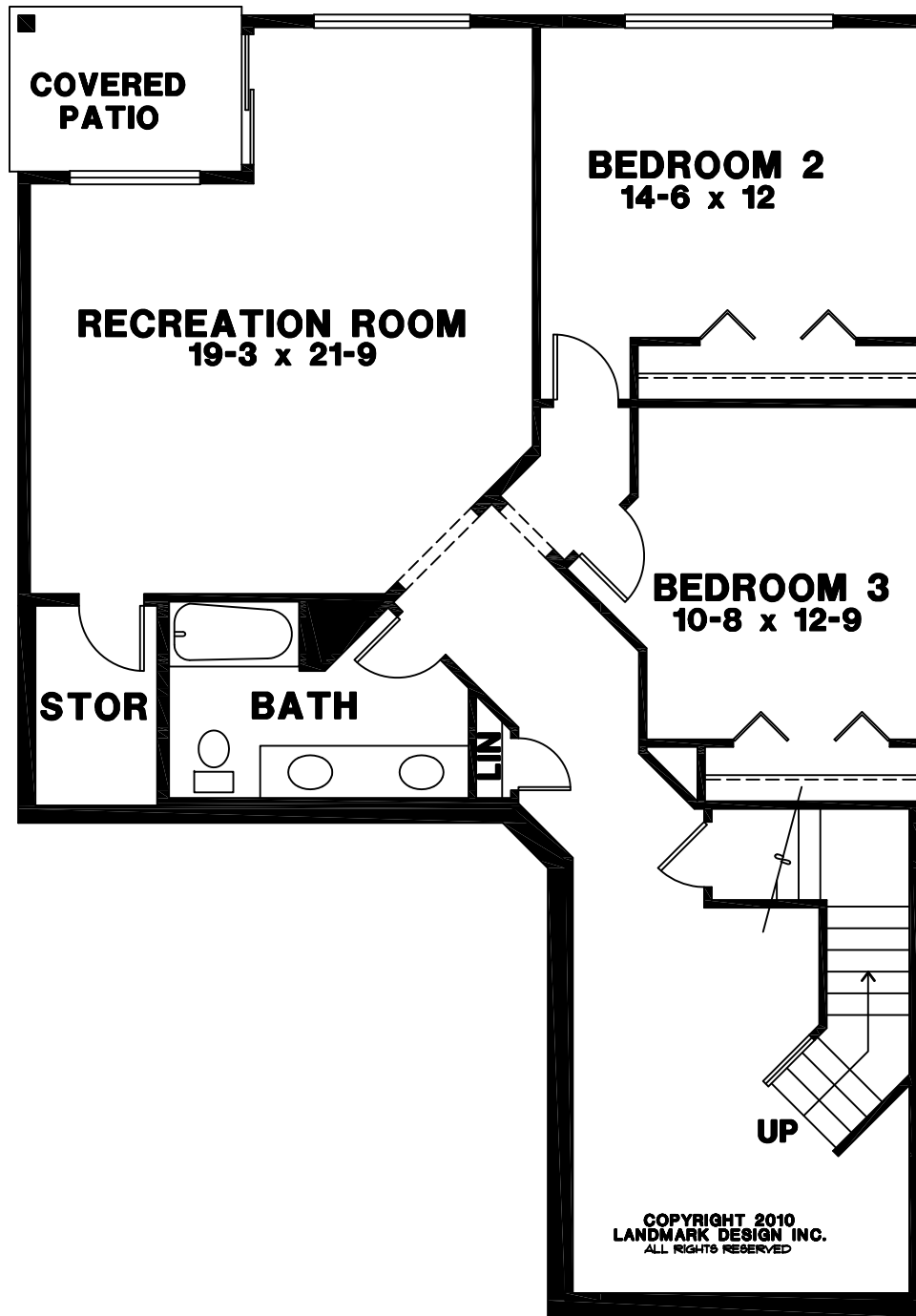
LOWER FLOOR
