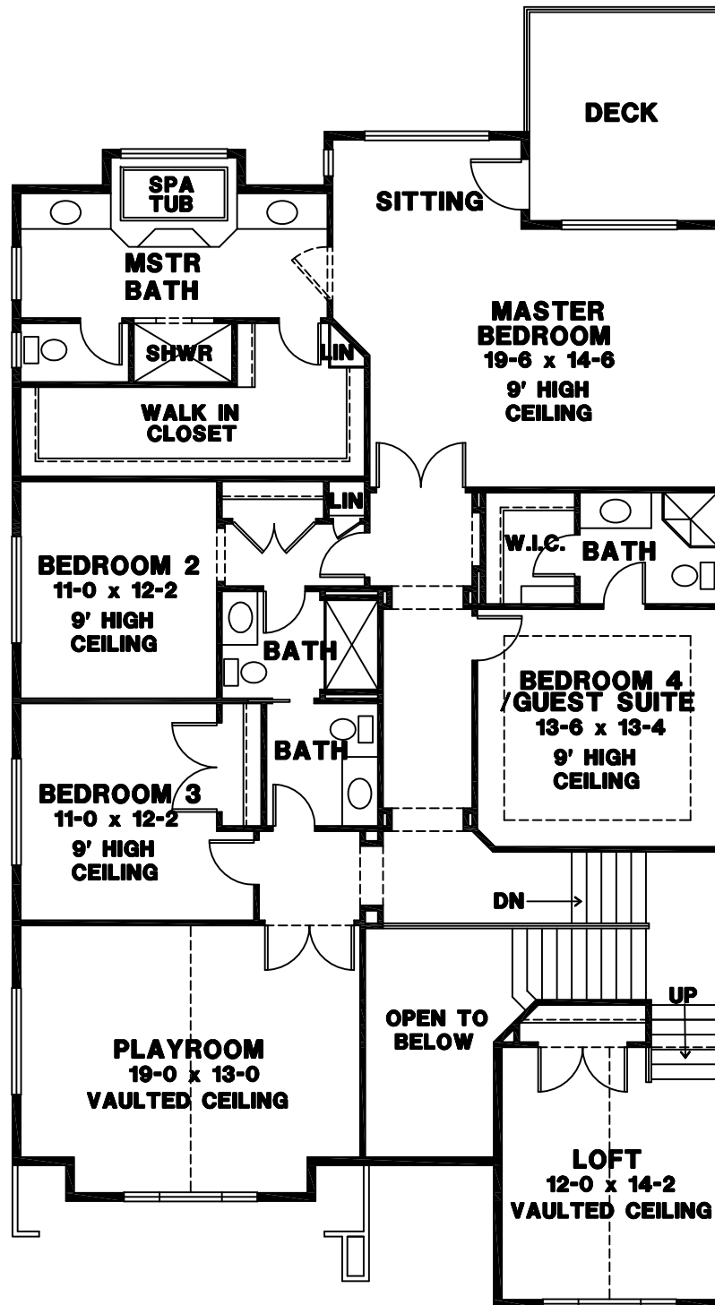
UPPER FLOOR
