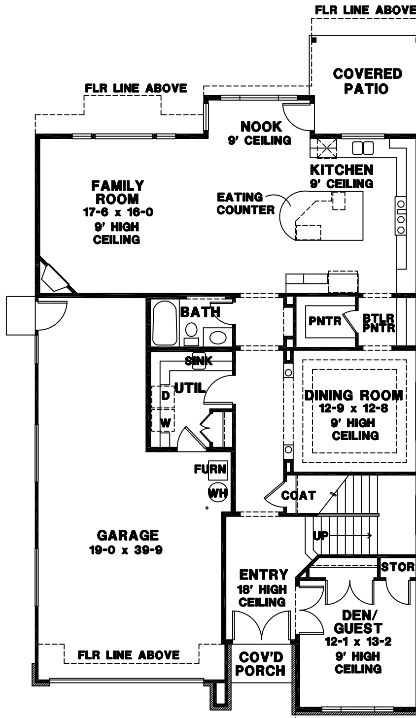
MAIN FLOOR
