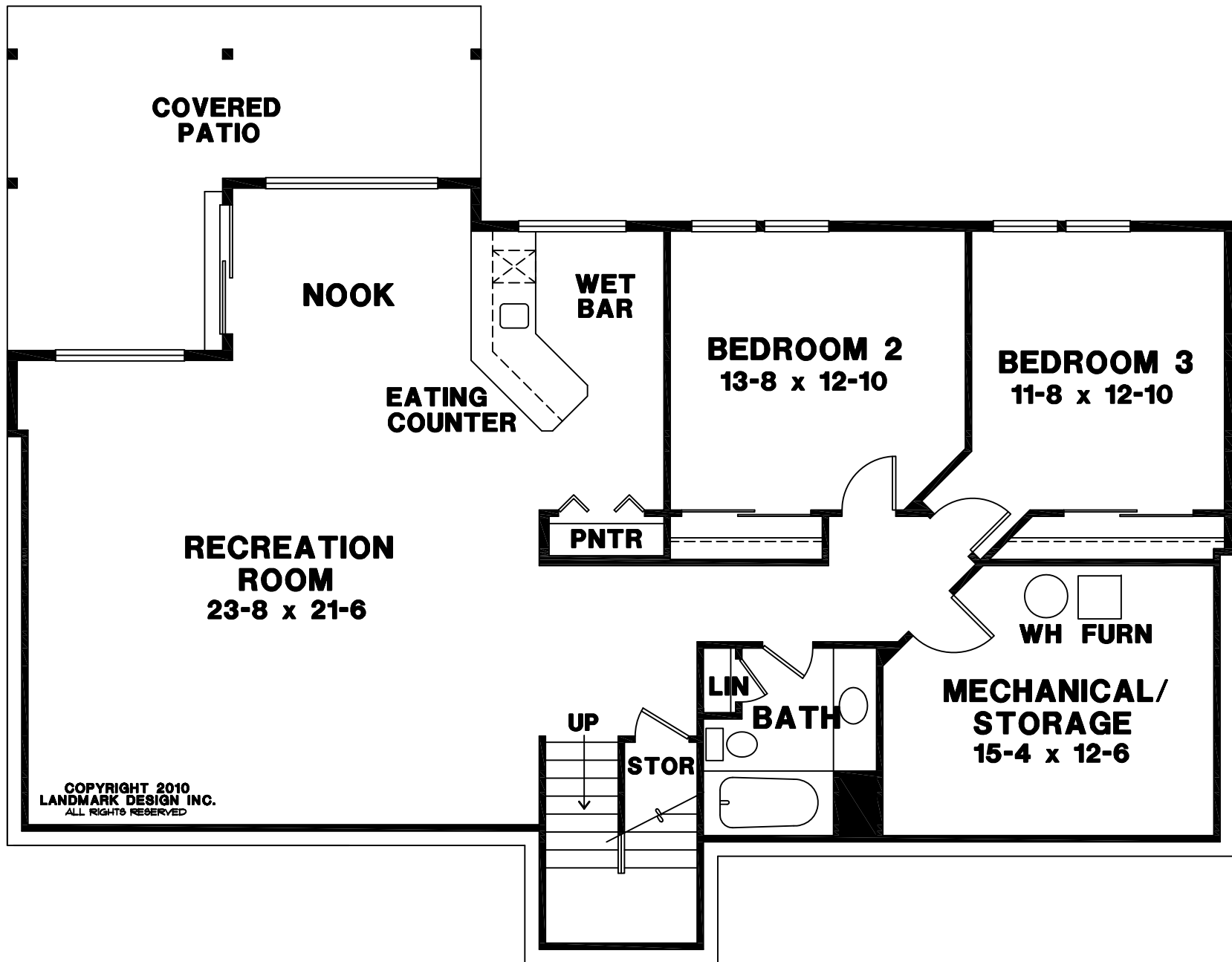
LOWER FLOOR
