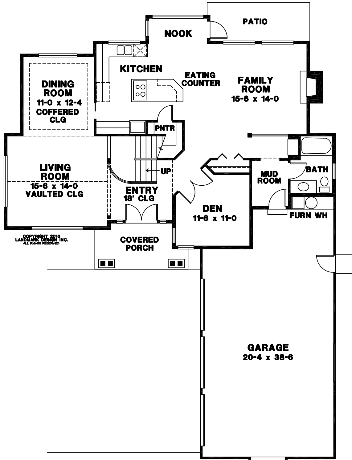
MAIN FLOOR
