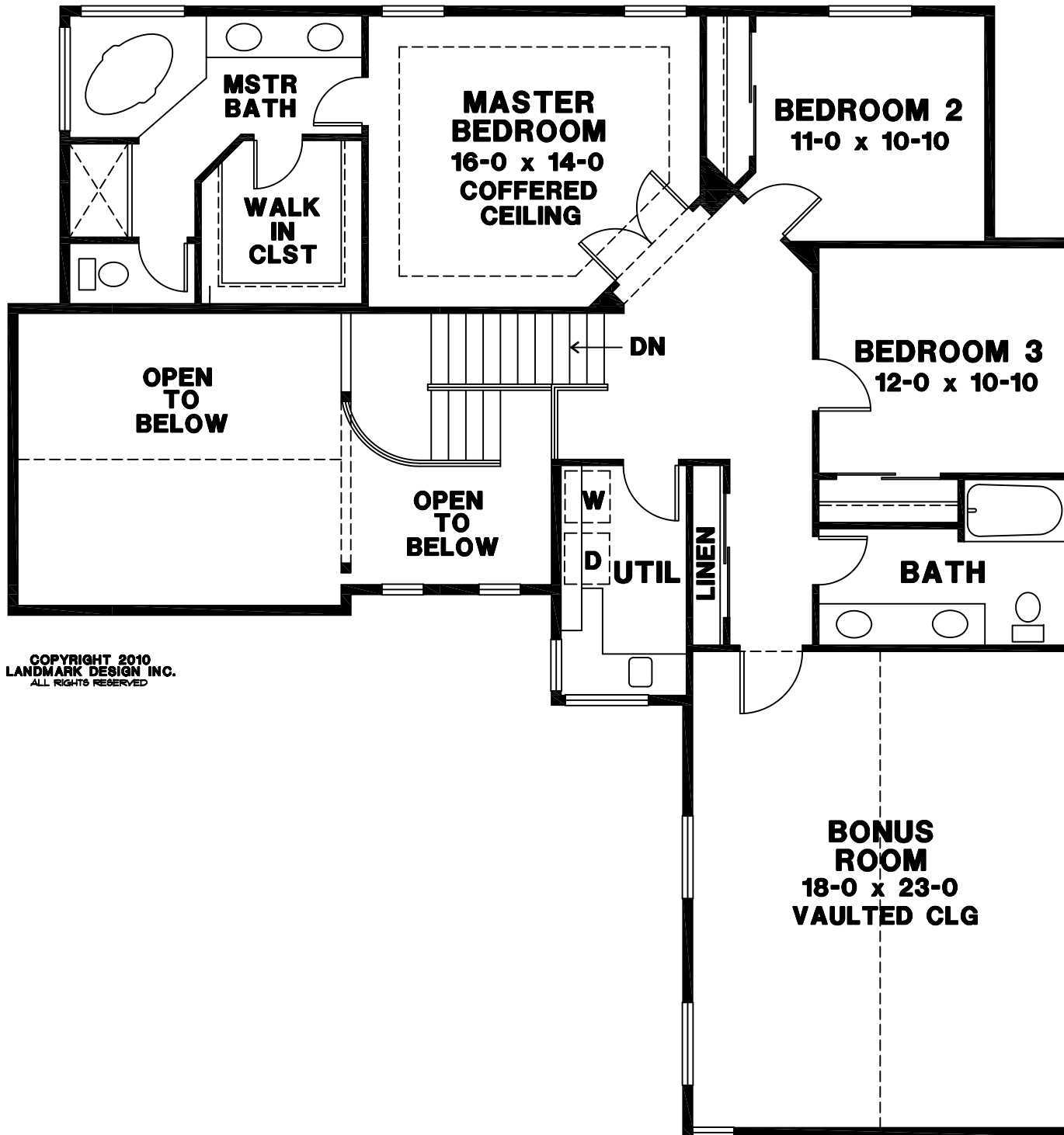
UPPER FLOOR
