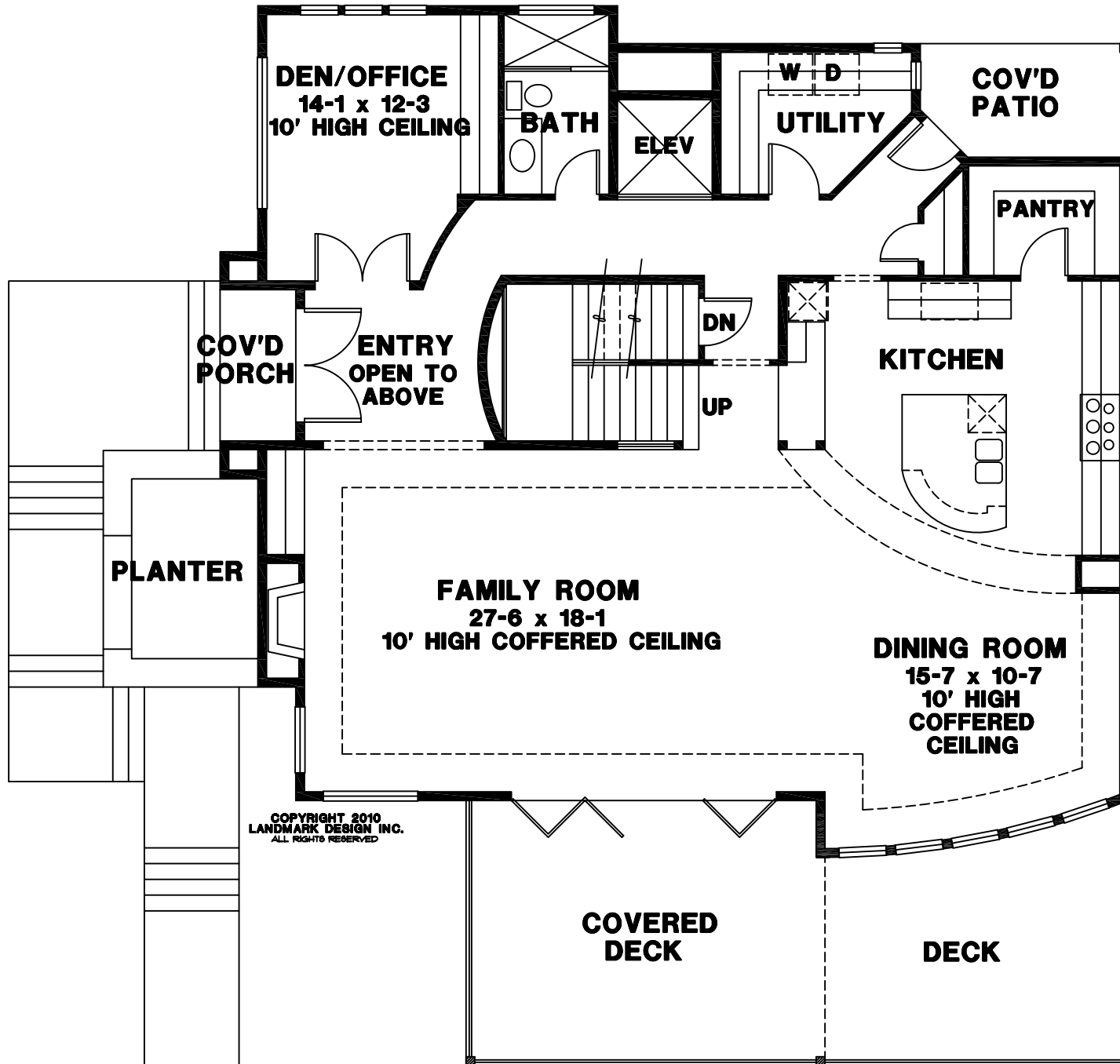
MAIN FLOOR
