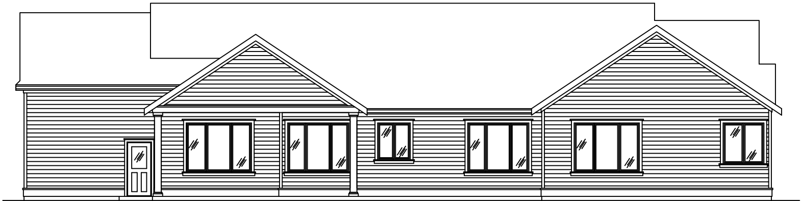
REAR ELEVATION
